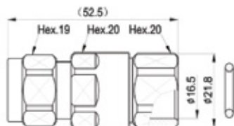
N Straight male Connector for 1/2" Flexible RF Cable
