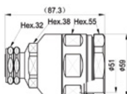
7/16 Straight male Connector for 1-5/8" Flexible RF Cable
