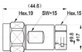
N Straight male Connector for 1/4" Flexible RF Cable
