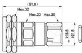
7/16 Straight male Connector for 1/2" Flexible RF Cable
