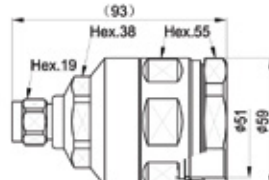
N Straight male Connector for 1-5/8" Flexible RF Cable
