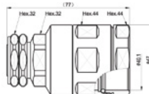
7/16 Straight male Connector for 1-1/4" Flexible RF Cable
